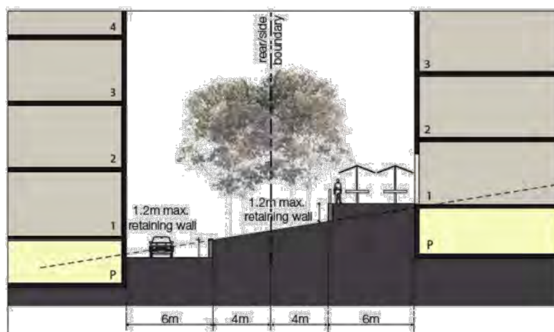
Figure 8.4.2 Level change controls at side and rear setbacks.
