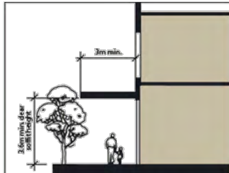
Figure 7.4.1 Awnings: Section
